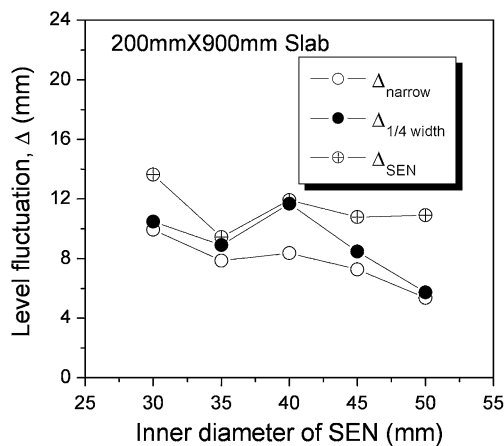
Fig. 16—Effect of inner bore diameter of SEN on level fluctuations in the mold.
