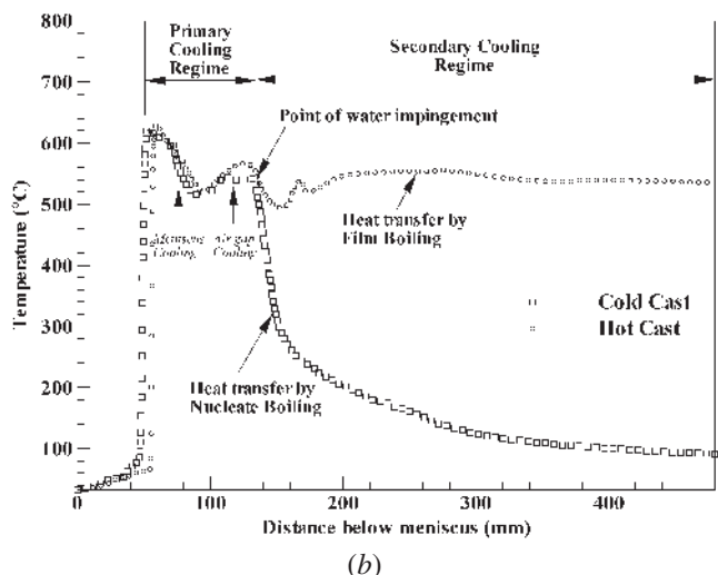
Fig. 13—Typical surface temperature profile and cooling regimes along strand length during continuous casting of (a) steel [25] and (b) aluminum [51] .
