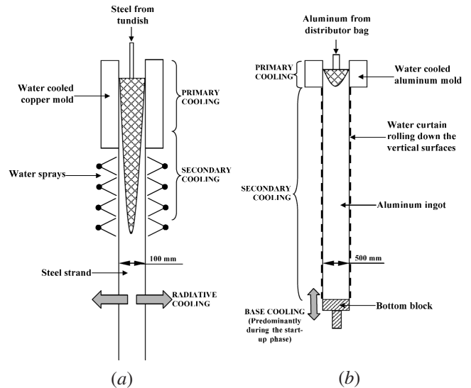
Fig. 2—Schematic of cooling processes, for (a) continuous casting of steel [15] and (b) DC casting of aluminum [5] .
