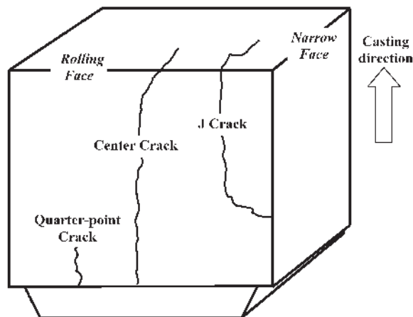
Fig. 15—Schematic of cold crack defects related to secondary cooling during DC casting of aluminum. [55]
