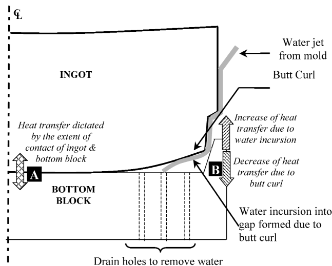
Fig. 12—Cooling and deformation of ingot base during the startup of DC casting, showing high contact near the center of the ingot (region A) and entry of secondary cooling water near the outer edges (region B). [5]
