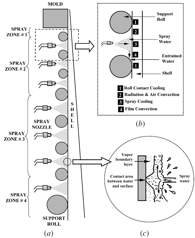
Fig. 8—Secondary cooling during continuous casting of steel: (a) typical arrangement of spray nozzles and support rolls, [45] (b) schematic of zones [25] , and (c) detail of water spray-cooling process [47] .
