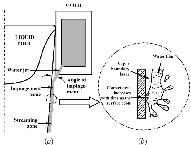
Fig. 9—(a) Secondary cooling regimes during DC casting of aluminum. [21] (b) Detail of water film cooling process. [47]
