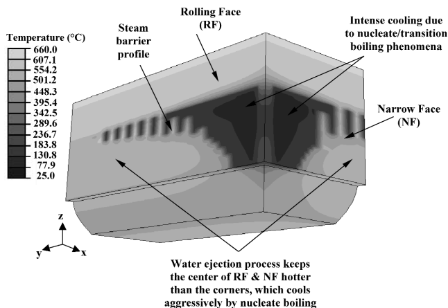
Fig. 21—Surface temperature contours on the narrow and rolling faces of a DC cast aluminum ingot at \sim 375 s after startup. [2,5,82]
