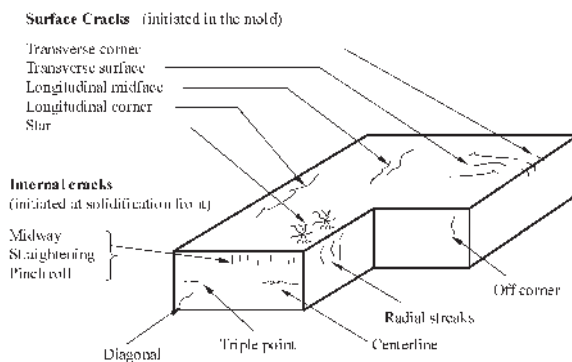
Fig. 14—Schematic of crack defects in continuous casting of steel. [54]
