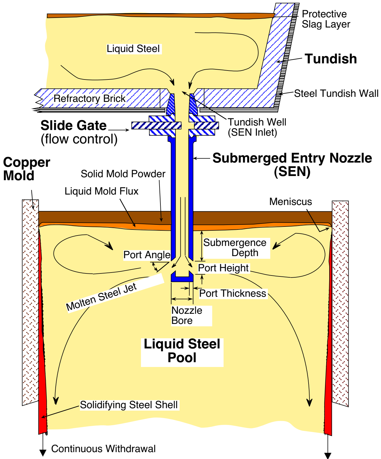
Figure 2. Schematic of mold region of continuous casting process for steel slabs
